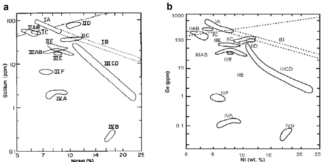
Fig. 7. Plot of Ge and Ga versus Ni for the studied meteorite, which is genetically quite similar to IIC subgroup or IIAB group.
